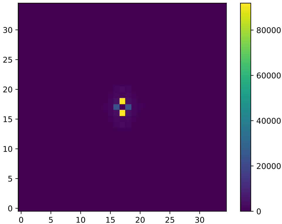
2D Structure Factor S(k) : T=0.46 , L=35
