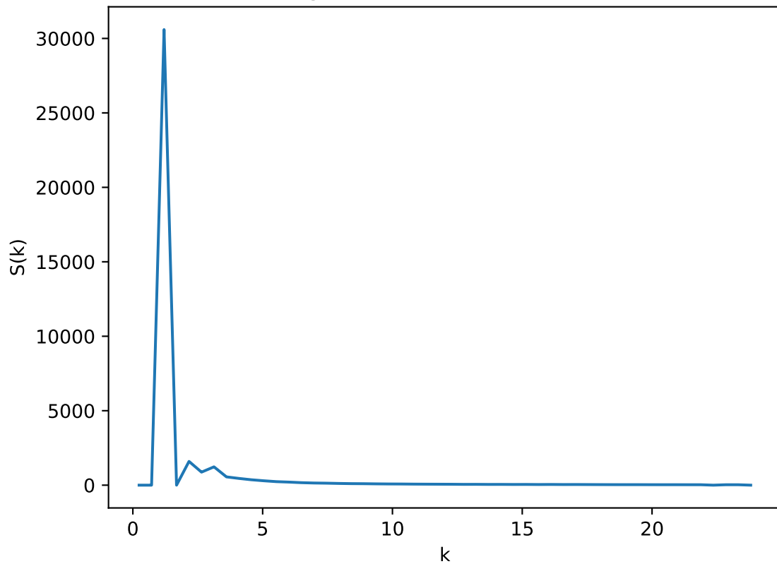
Radial Average of Structure Factor: T=0.46 , L=35
