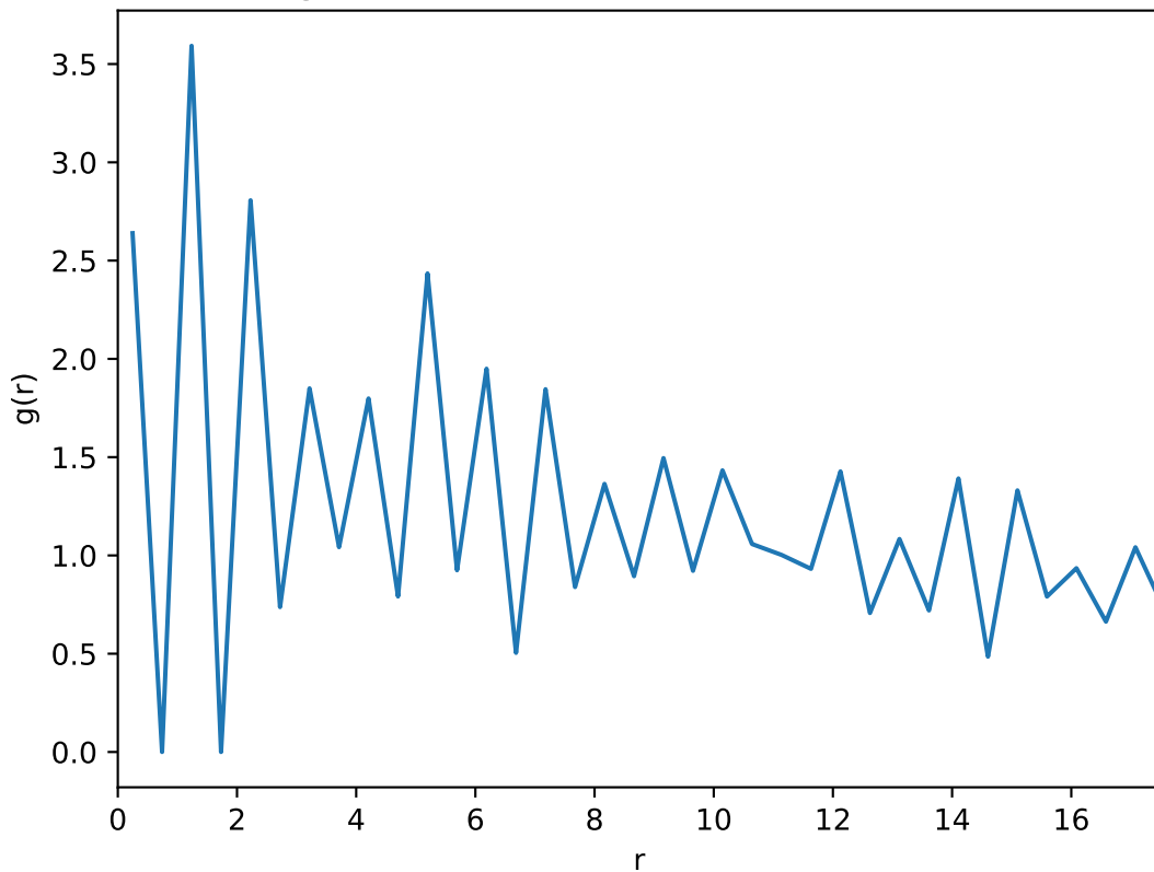
Average radial distribution function: T=0.52 , L=35
