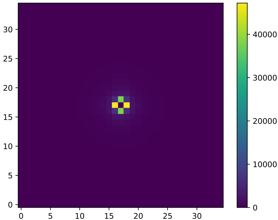
2D Structure Factor S(k) : T=0.52 , L=35
