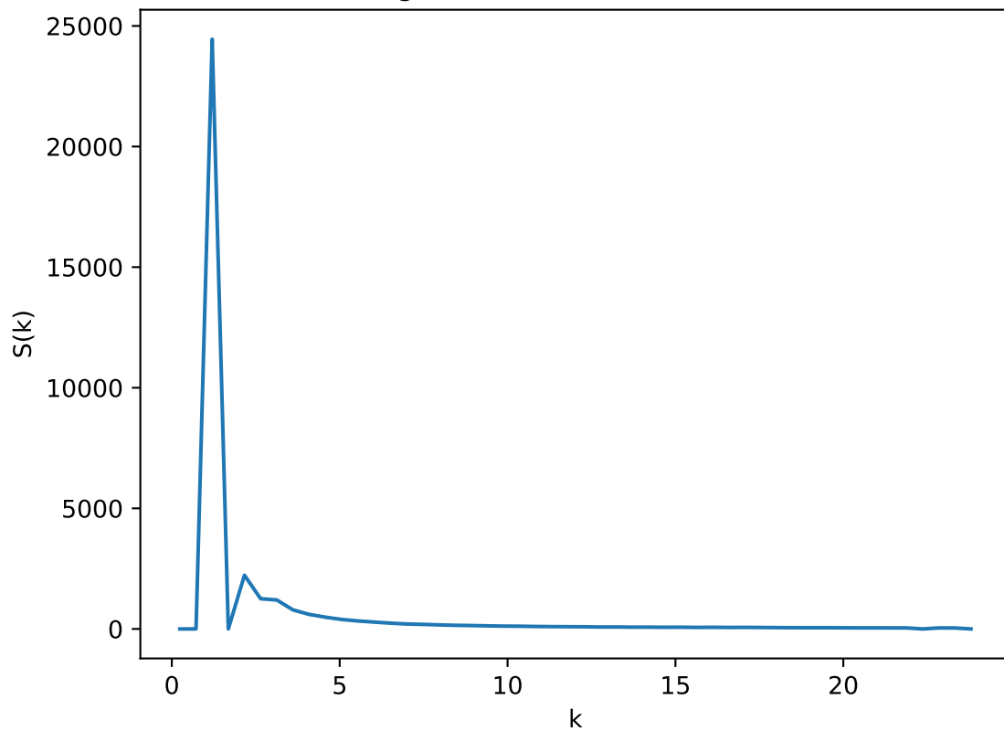
Radial Average of Structure Factor: T=0.52 , L=35
