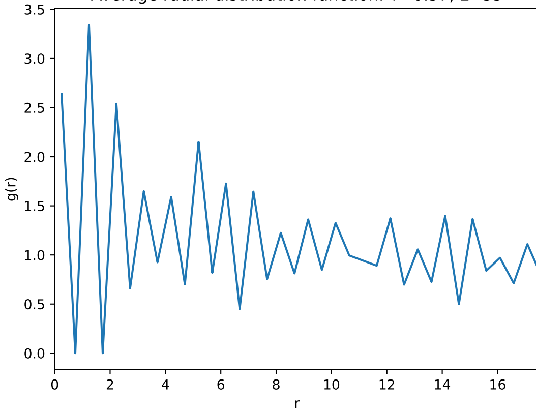
Average radial distribution function: T=0.57 , L=35
