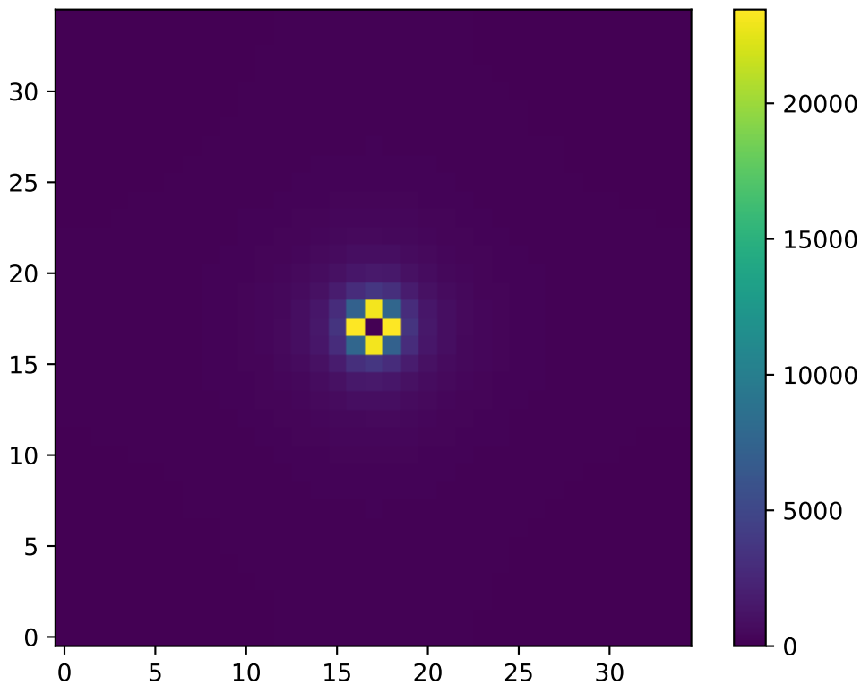
2D Structure Factor S(k) : T=0.57 , L=35
