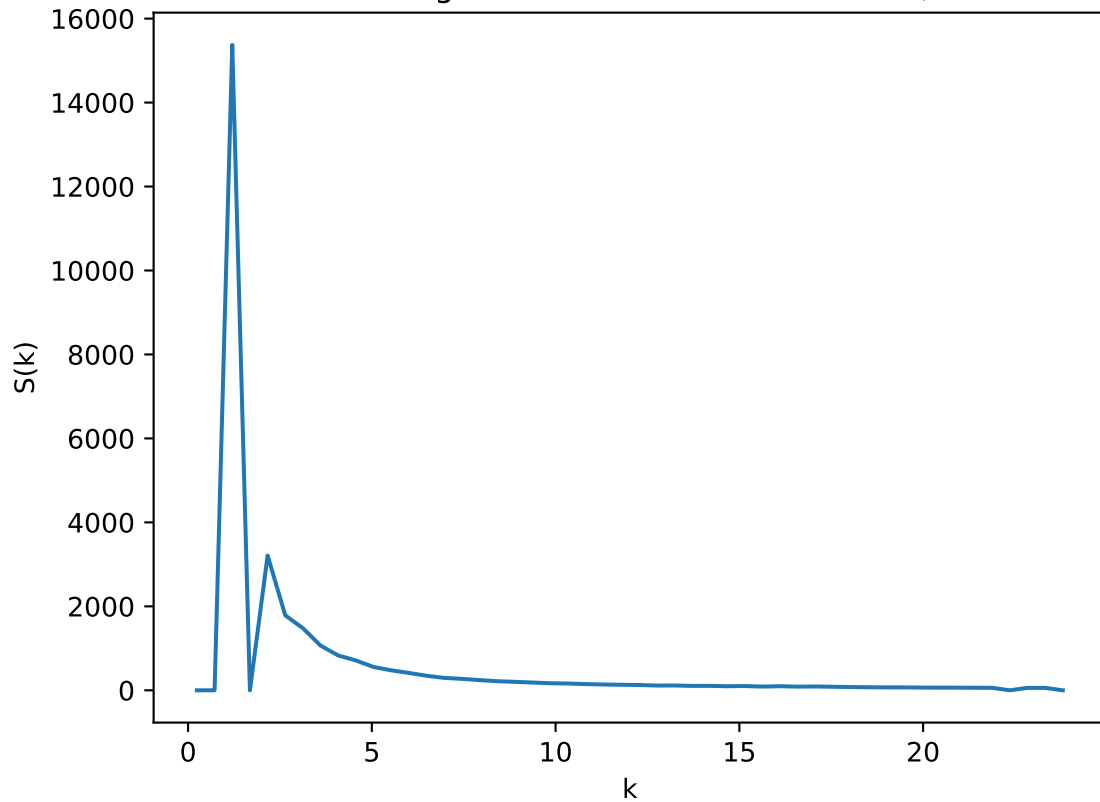
Radial Average of Structure Factor: T=0.57 , L=35
