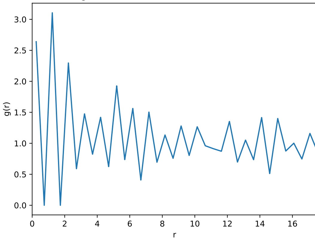
Average radial distribution function: T=0.63 , L=35
