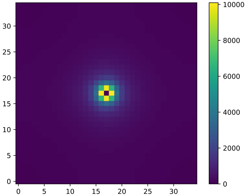
2D Structure Factor S(k) : T=0.63 , L=35
