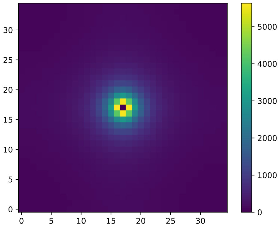
2D Structure Factor S(k) : T=0.68 , L=35
