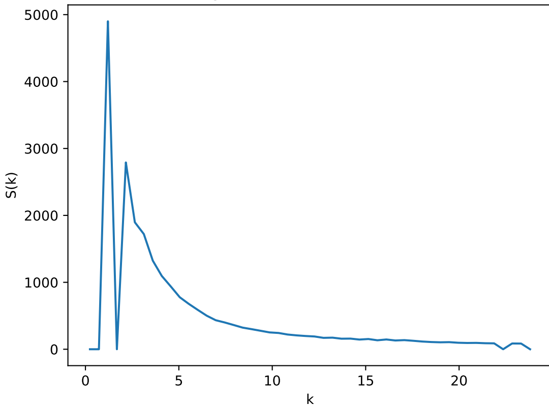
Radial Average of Structure Factor: T=0.68 , L=35
