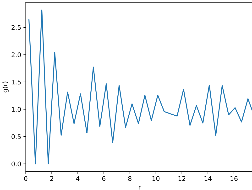
Average radial distribution function: T=0.74 , L=35
