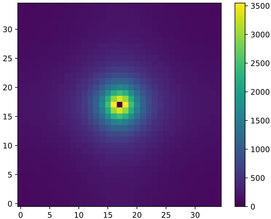
2D Structure Factor S(k) : T=0.74 , L=35
