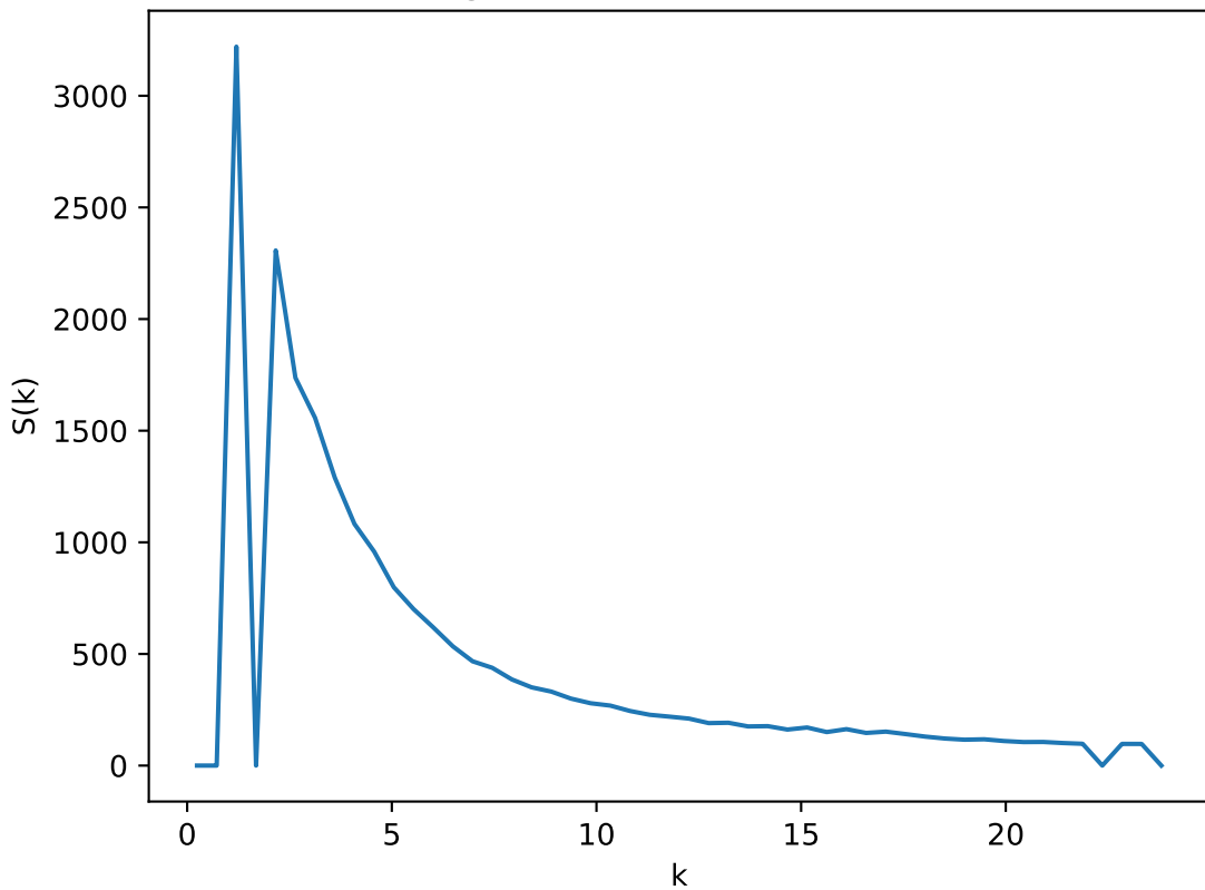
Radial Average of Structure Factor: T=0.74 , L=35
