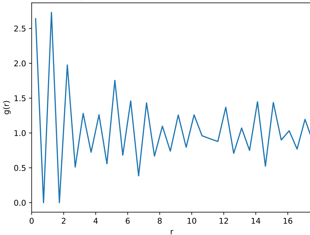
Average radial distribution function: T=0.79 , L=35
