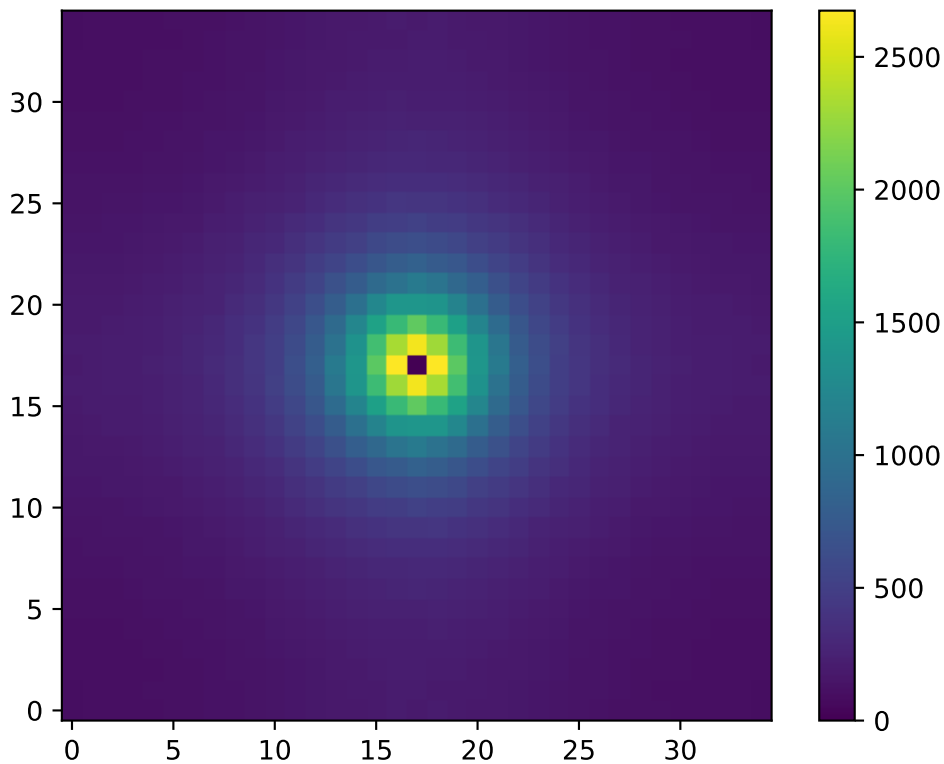
2D Structure Factor S(k) : T=0.79 , L=35
