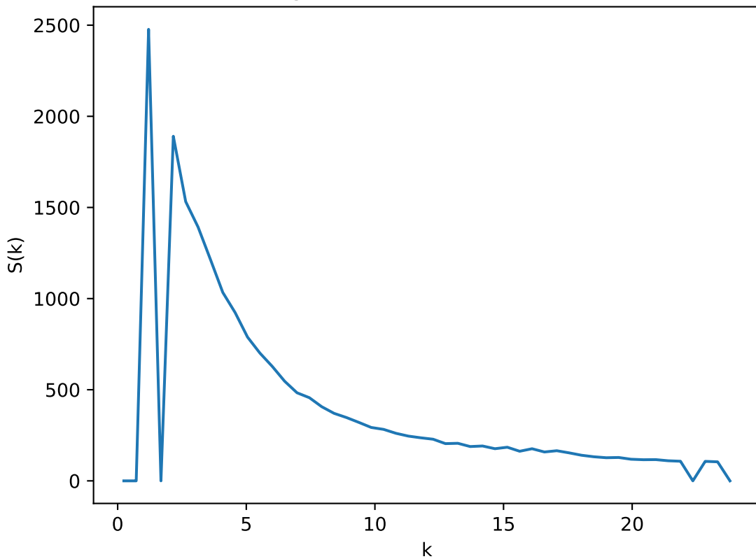
Radial Average of Structure Factor: T=0.79 , L=35
