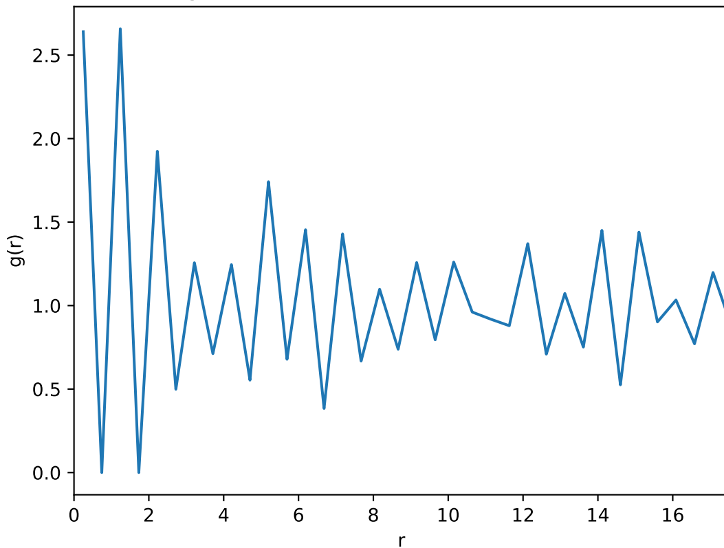
Average radial distribution function: T=0.85 , L=35
