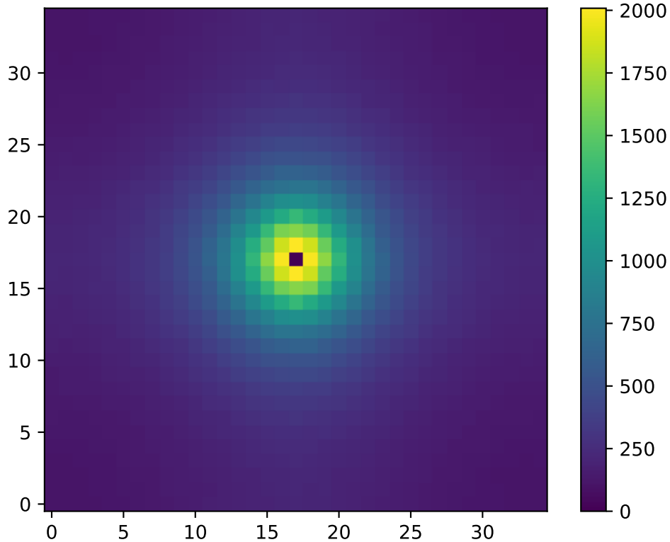
2D Structure Factor S(k) : T=0.85 , L=35
