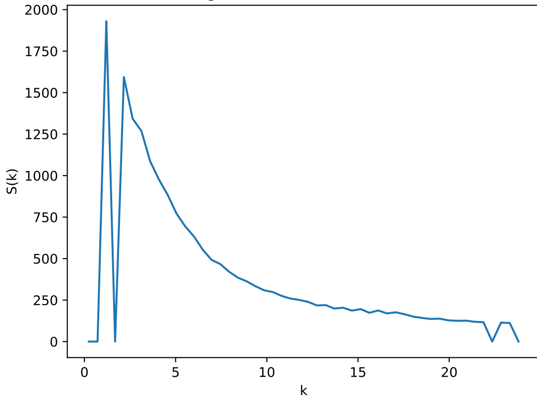
Radial Average of Structure Factor: T=0.85 , L=35
