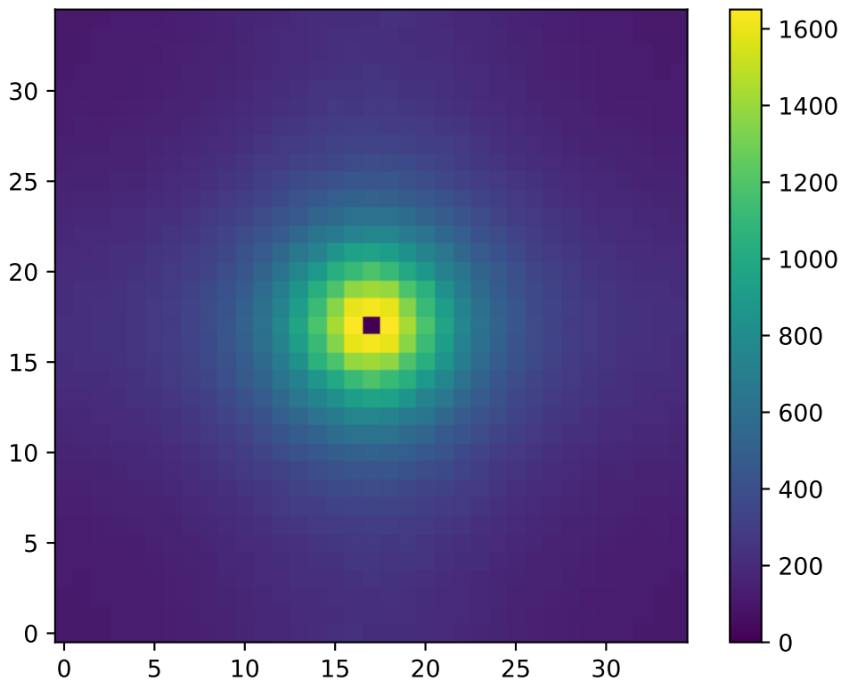
2D Structure Factor S(k) : T=0.90 , L=35
