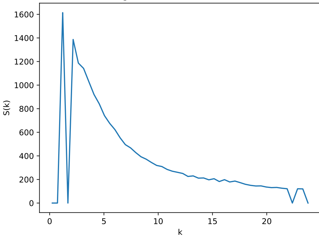
Radial Average of Structure Factor: T=0.90 , L=35
