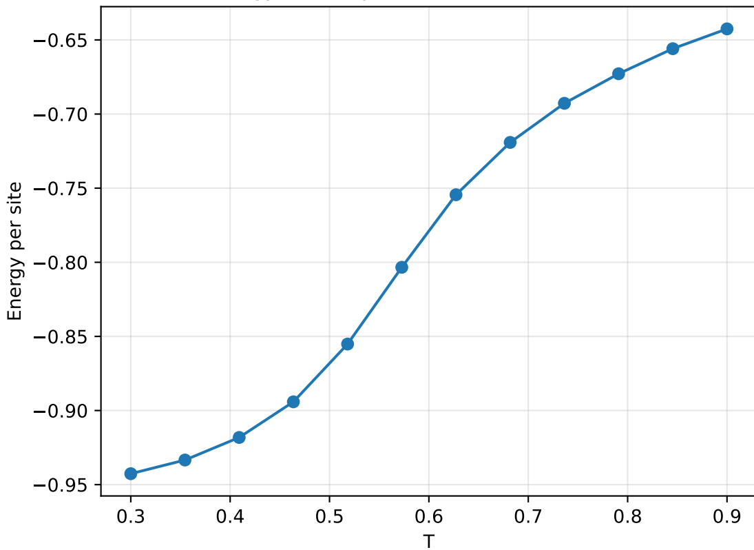
Energy vs Temperature ( L=35 , \rho=0.50 )
