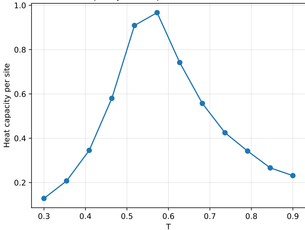
Heat Capacity vs Temperature ( L=35 , \rho=0.50 )
