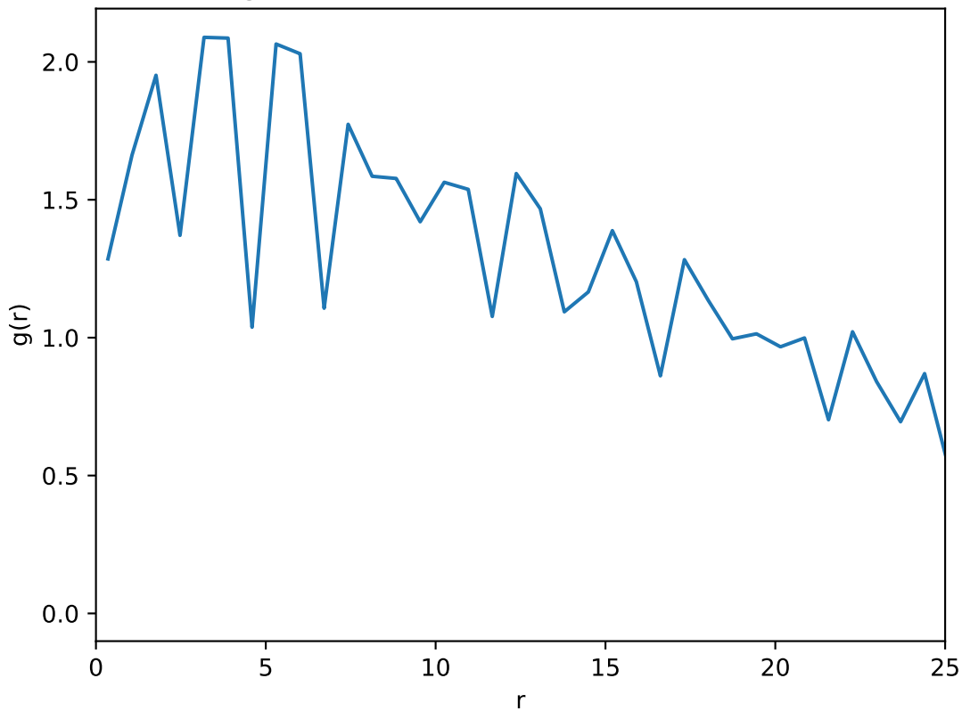
Average radial distribution function: T=0.30 , L=50
