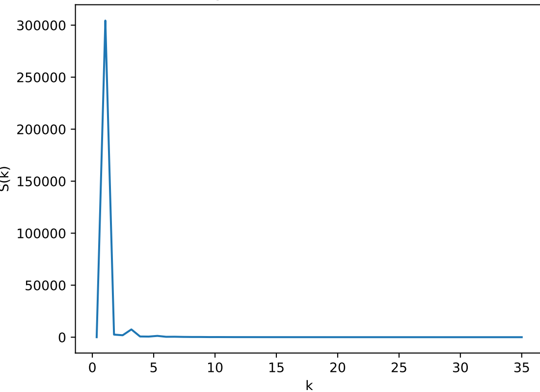
Radial Average of Structure Factor: T=0.30 , L=50
