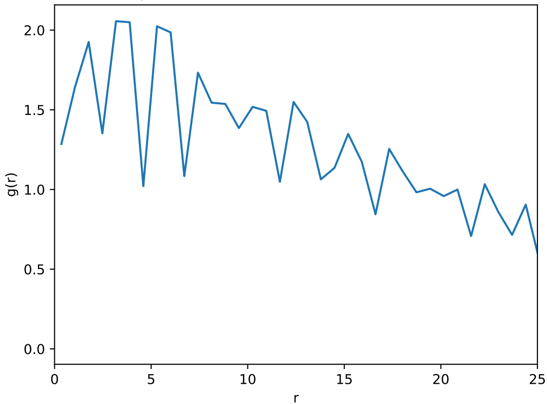
Average radial distribution function: T=0.35 , L=50
