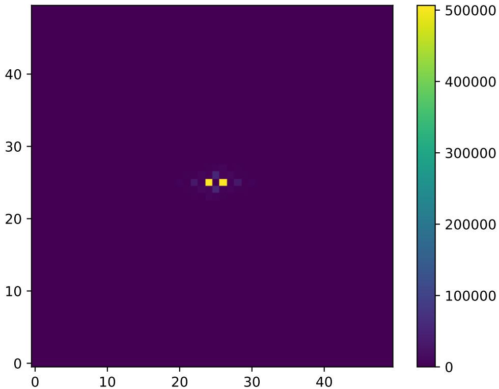
2D Structure Factor S(k) : T=0.35 , L=50
