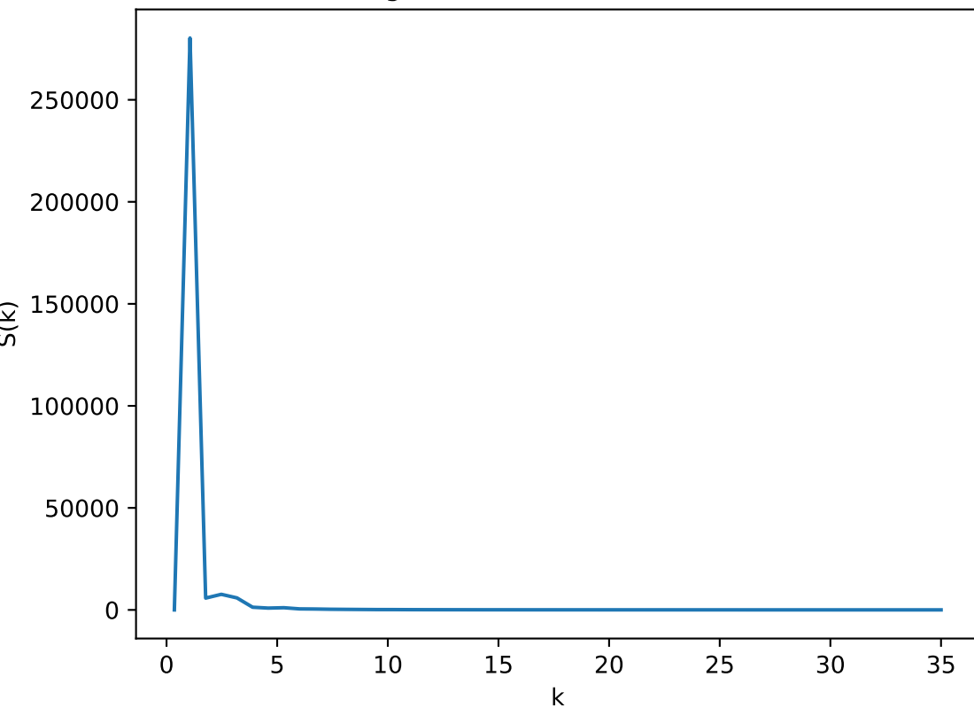
Radial Average of Structure Factor: T=0.35 , L=50
