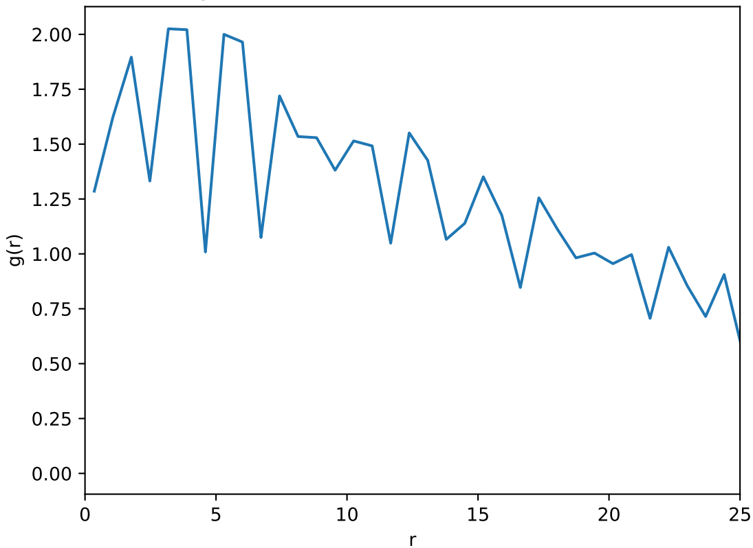
Average radial distribution function: T=0.41 , L=50
