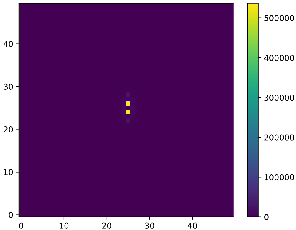
2D Structure Factor S(k) : T=0.41 , L=50
