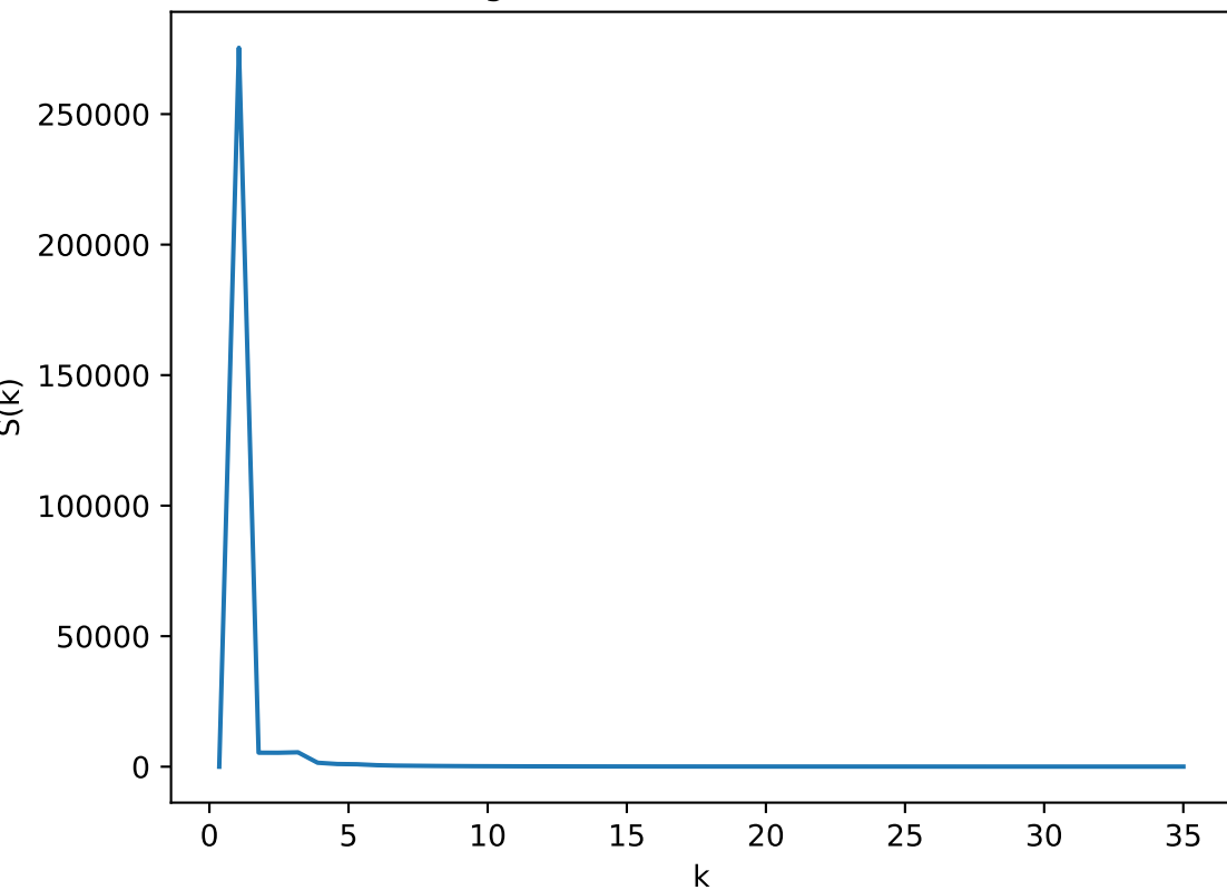
Radial Average of Structure Factor: T=0.41 , L=50
