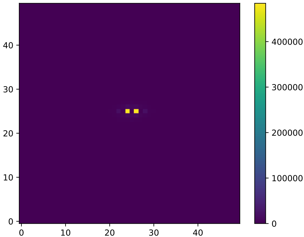
2D Structure Factor S(k) : T=0.46 , L=50
