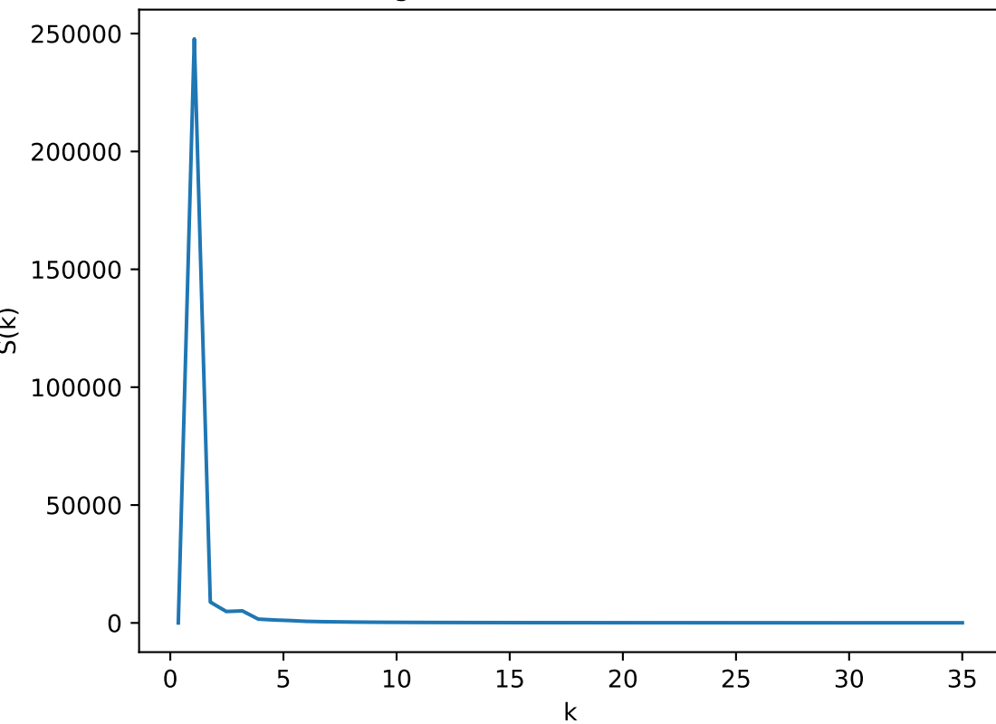
Radial Average of Structure Factor: T=0.46 , L=50
