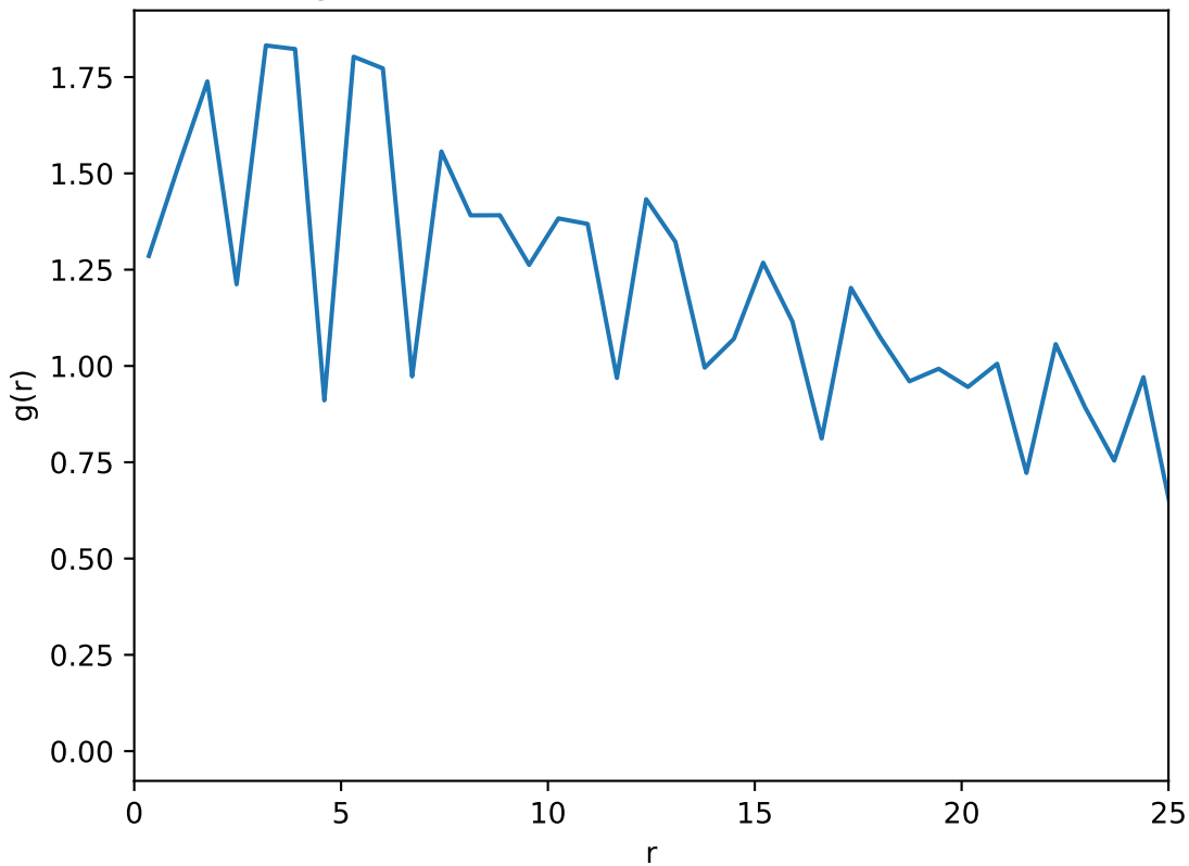
Average radial distribution function: T=0.52 , L=50
