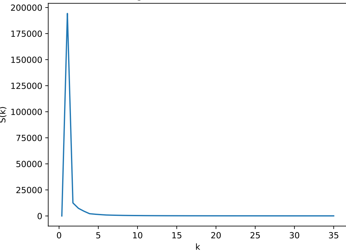
Radial Average of Structure Factor: T=0.52 , L=50
