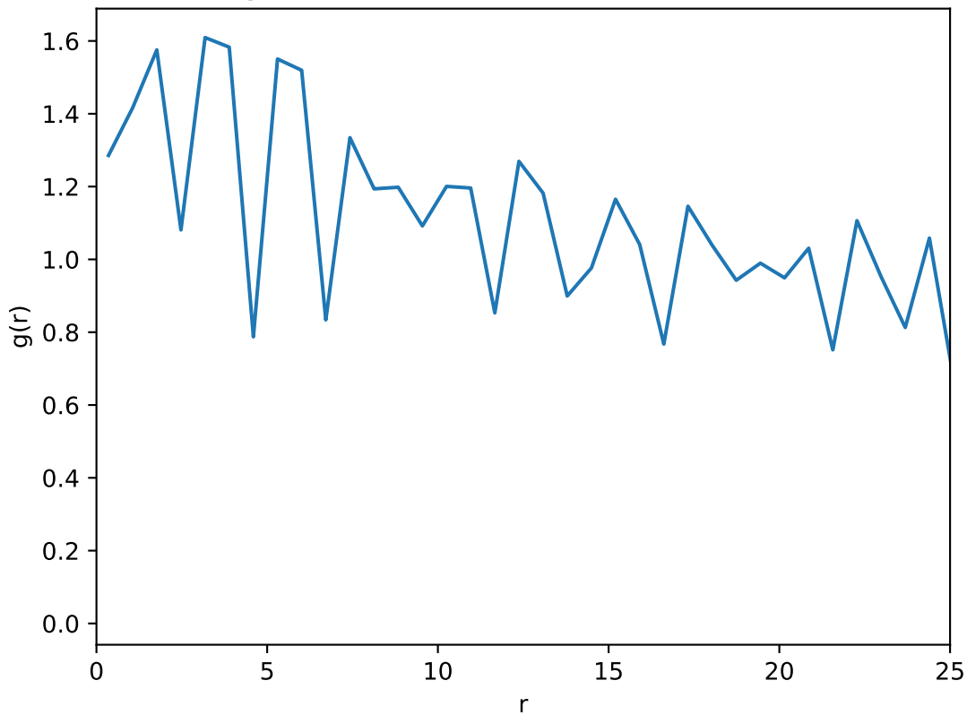
Average radial distribution function: T=0.57 , L=50
