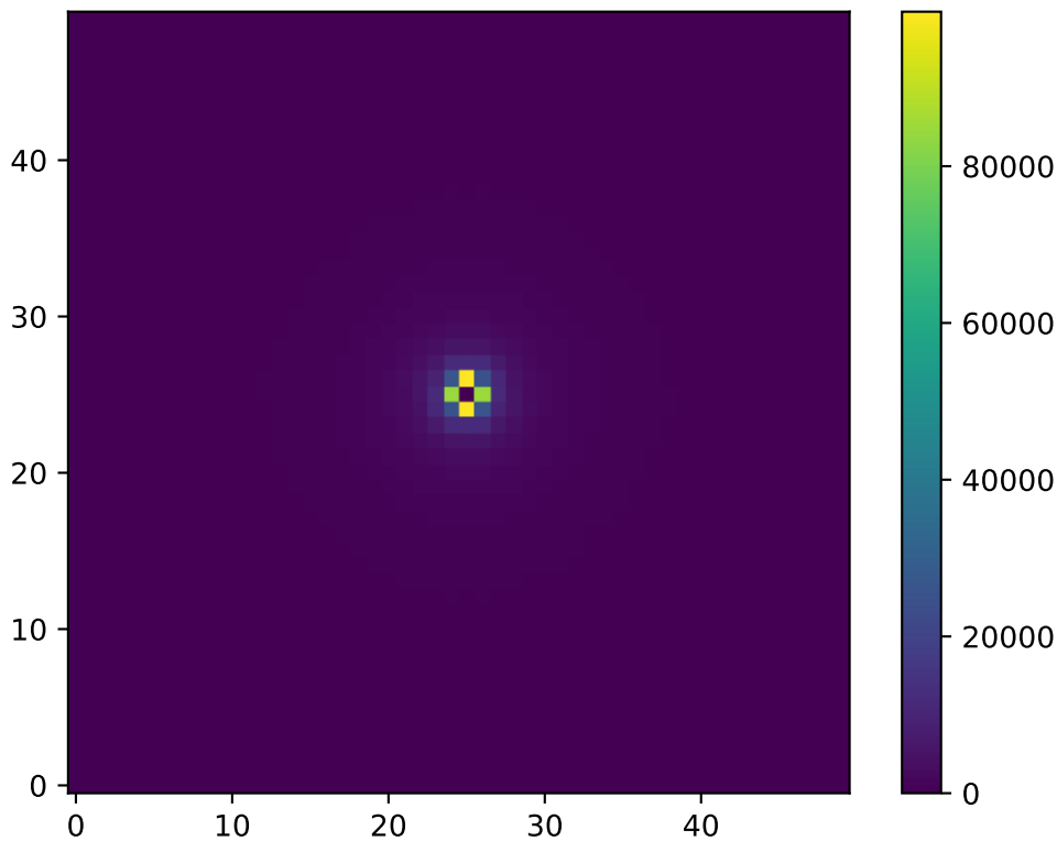
2D Structure Factor S(k) : T=0.57 , L=50
