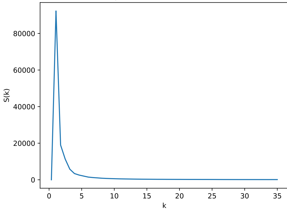
Radial Average of Structure Factor: T=0.57 , L=50
