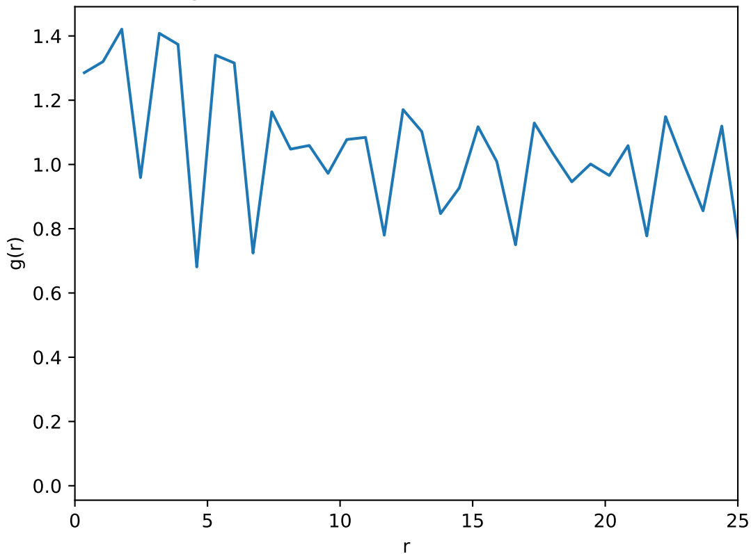
Average radial distribution function: T=0.63 , L=50
