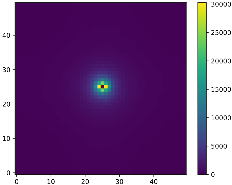
2D Structure Factor S(k) : T=0.63 , L=50
