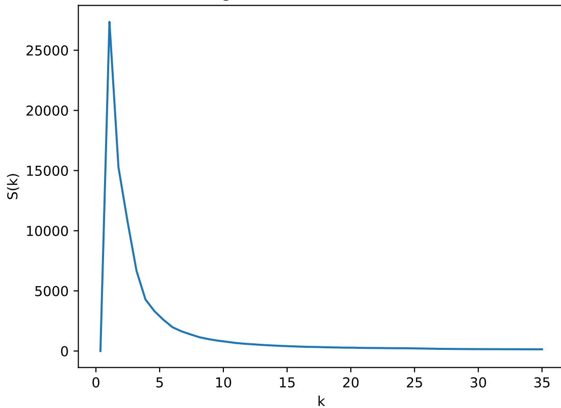
Radial Average of Structure Factor: T=0.63 , L=50
