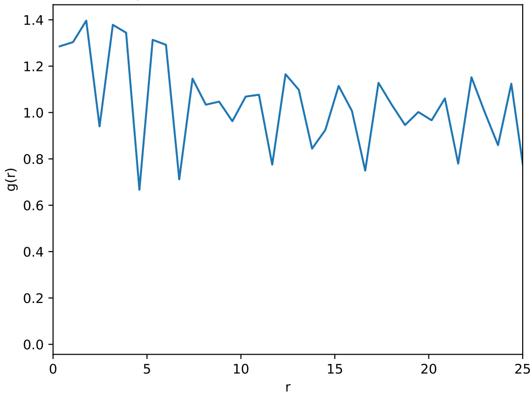
Average radial distribution function: T=0.64 , L=50
