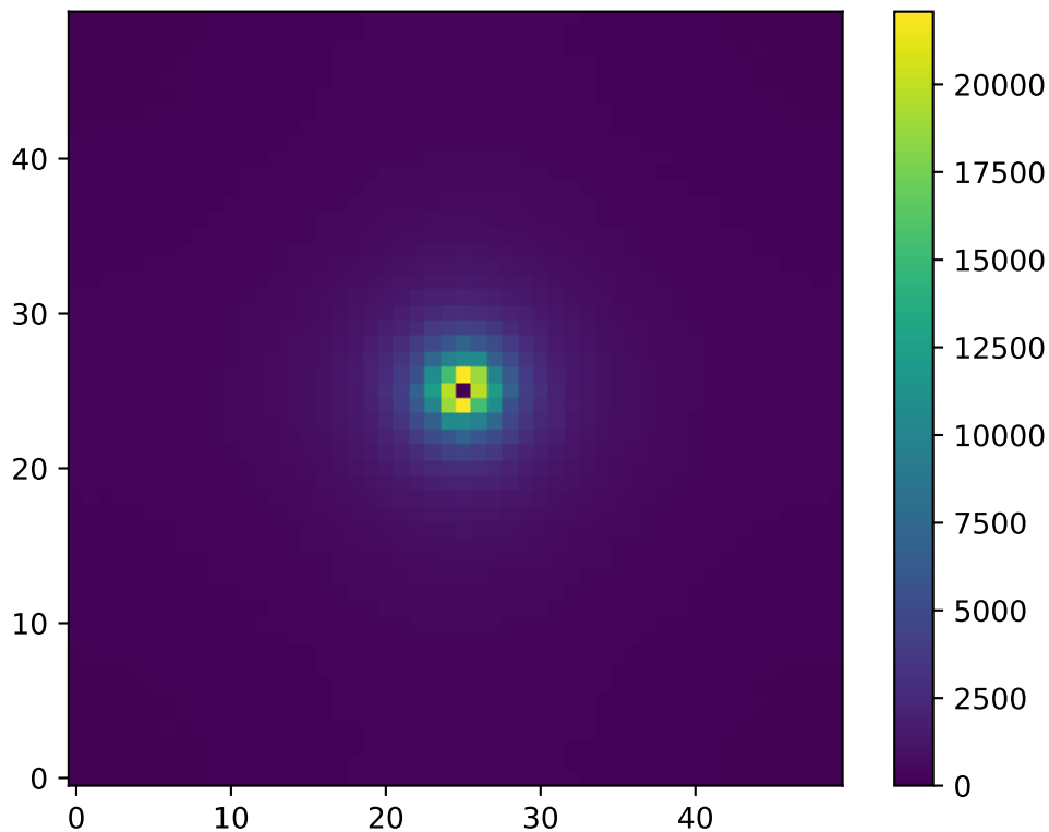
2D Structure Factor S(k) : T=0.64 , L=50
