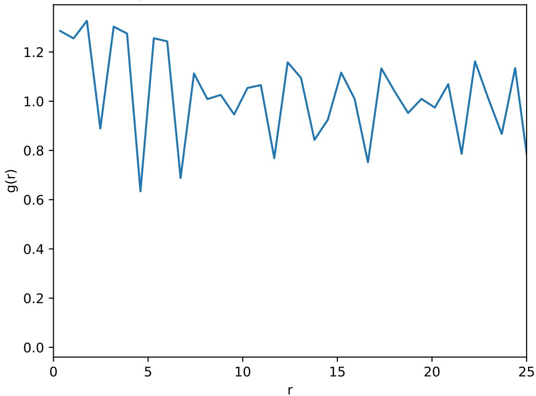
Average radial distribution function: T=0.68 , L=50
