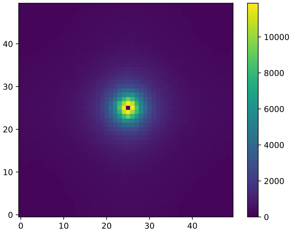
2D Structure Factor S(k) : T=0.68 , L=50
