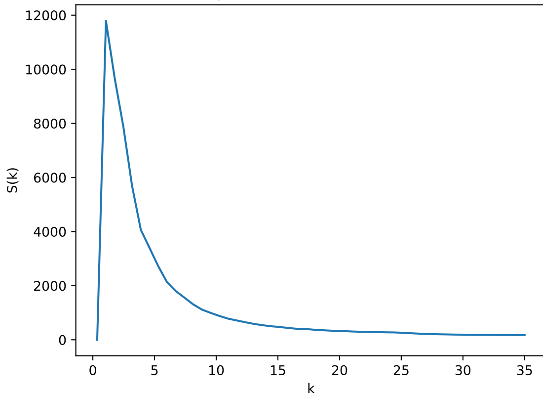
Radial Average of Structure Factor: T=0.68 , L=50
