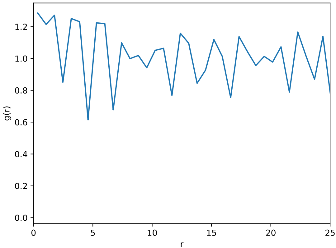
Average radial distribution function: T=0.73 , L=50
