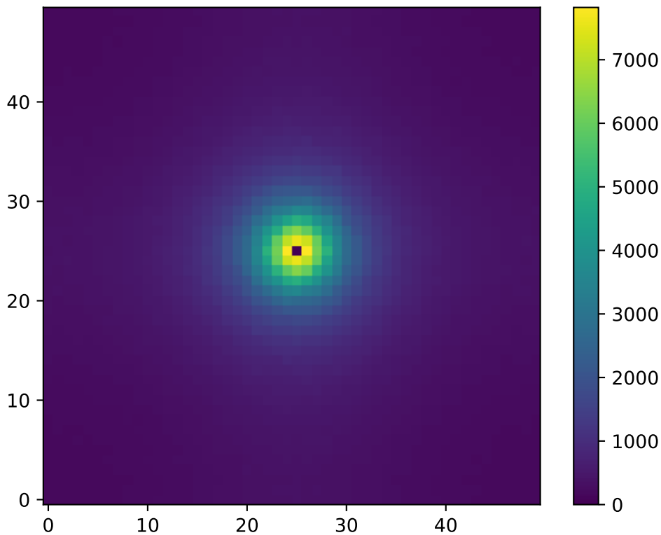
2D Structure Factor S(k) : T=0.73 , L=50
